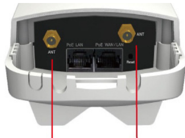
2xRP-SMA Female
